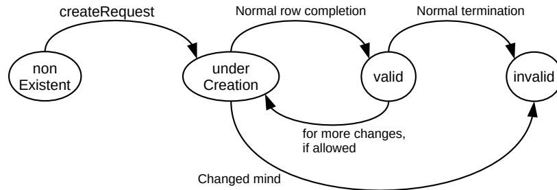
Transition diagram for EntryStatus. When a row is requested with createRequest, it is actually created as underCreation.
